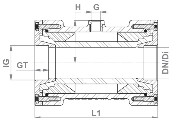
DN20 - DN25
